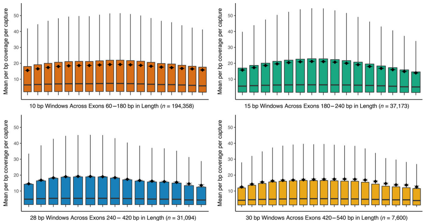
FIGURE 5 Boxplots of mean per basepair coverage levels plotted across exon size windows. All annotated exons were broken into 10–30 bp windows depending on overall size, and the mean per basepair coverage per capture was calculated for each window size. The line each box represents the median of mean coverage values and the box surrounds the 25th and 75th percentiles. The mean of each bin class is plotted as a black diamond with standard error bars around it. Outlier points were not plotted. Note that the data for this graph are for all annotated exons, regardless of expected capture. See Supporting Information Figure S3 for a similar plot focused on an expressed target set
